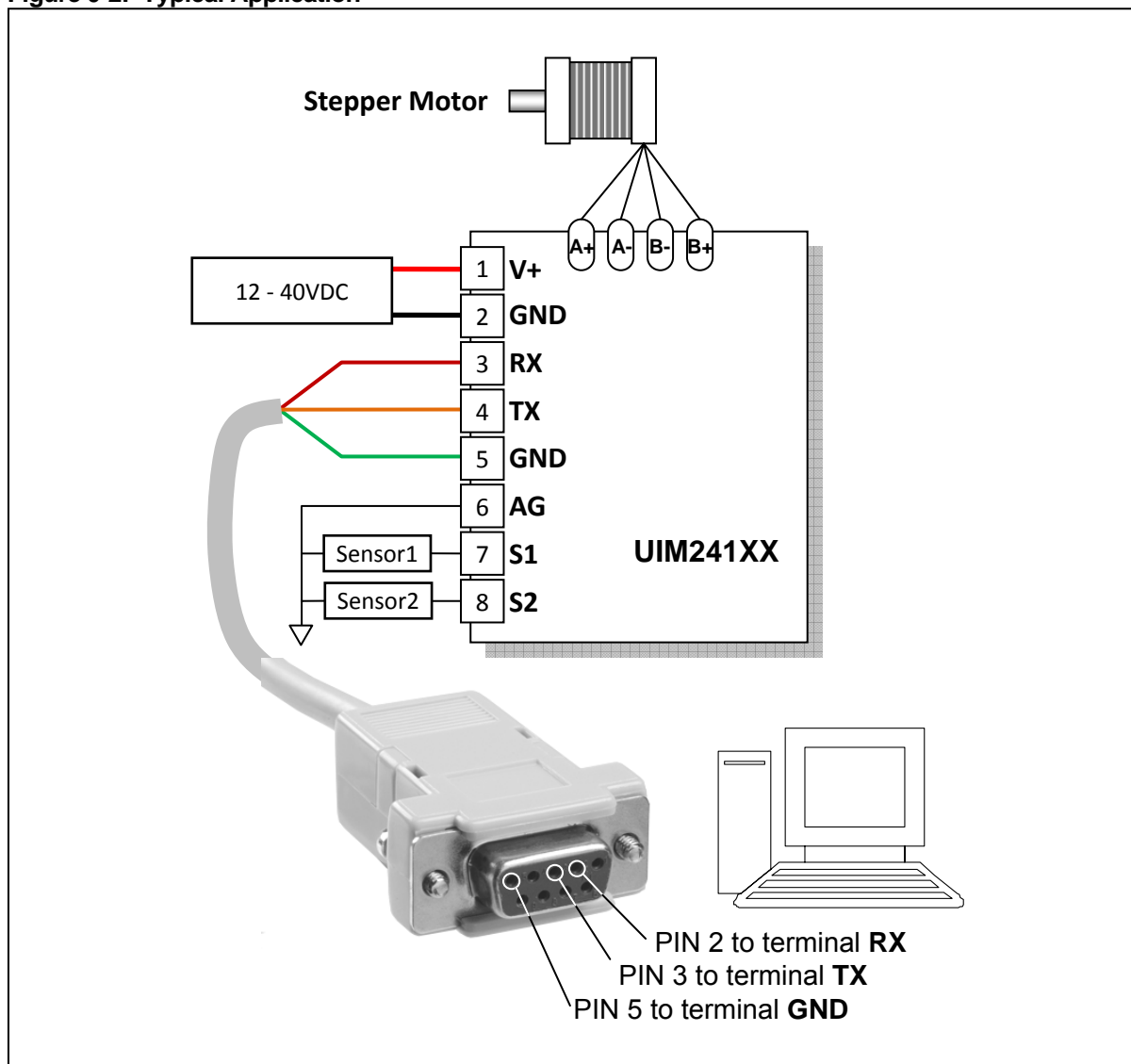
Figure 0-2: Typical Application
