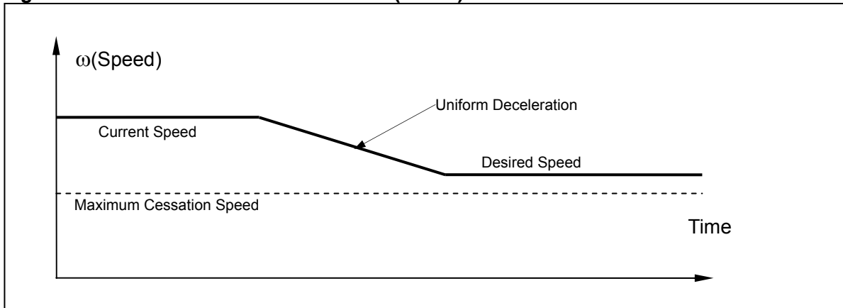
Figure 7-6: Nonlinear Deceleration Control (case 1)
