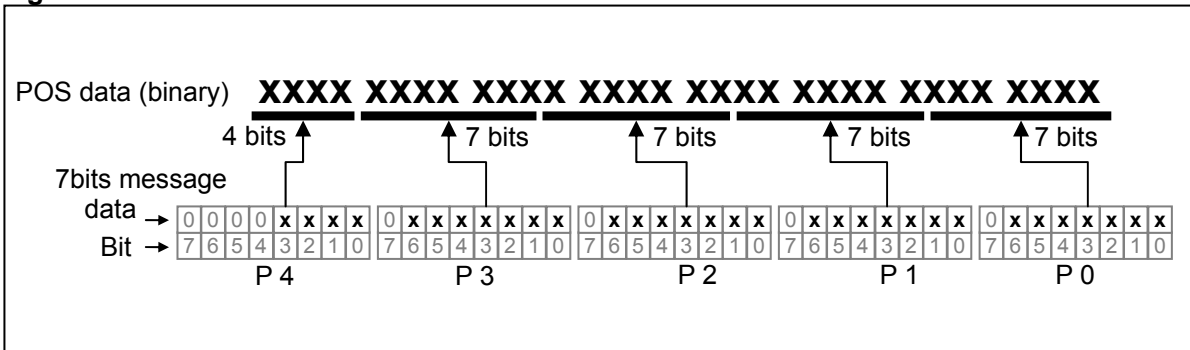
Figure 6-1: Conversion from P4:P0 to 32bits POS value
