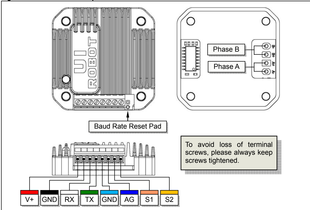
Figure 0-1: Terminal Description
