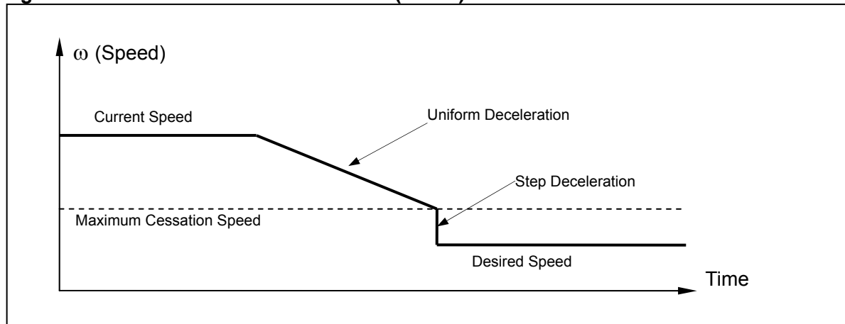
Figure 7-7: Nonlinear Deceleration Control (case 2)
